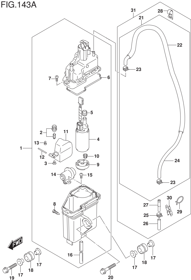
DF175_E01_018_143A FUEL VAPOR SEPARATOR
