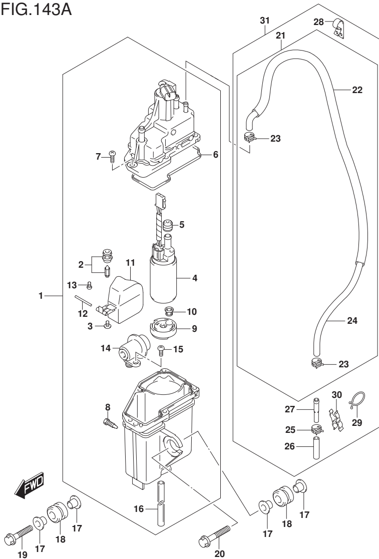
FIG.143A (1-C-6) FUEL VAPOR SEPARATOR (E01)
