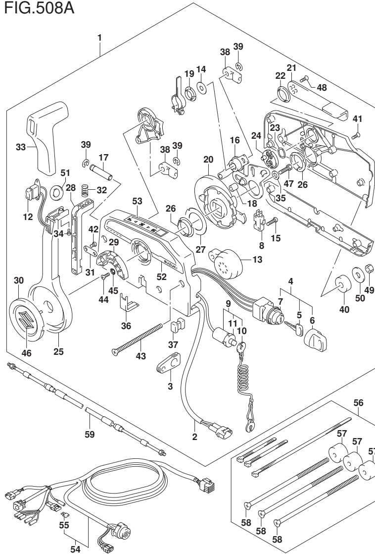
FIG.508A (1-G-12) OPT:REMOTE CONTROL
