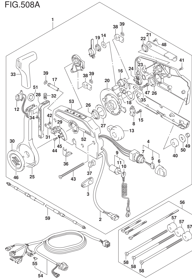
FIG.508A (1-G-14) OPT:REMOTE CONTROL
