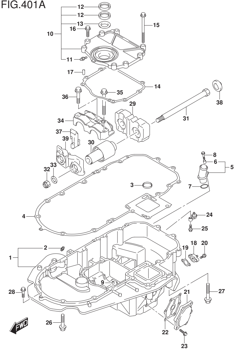
FIG.401A (1-F-5) ENGINE HOLDER
