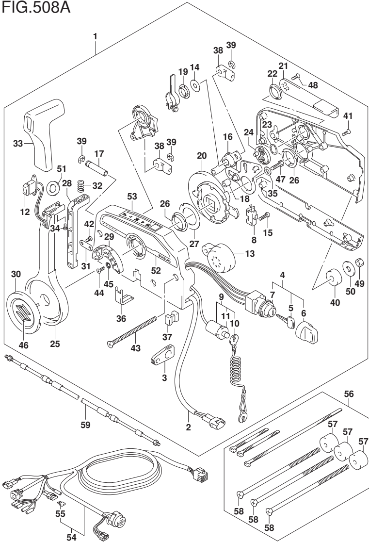
FIG.508A (1-G-13) OPT:REMOTE CONTROL
