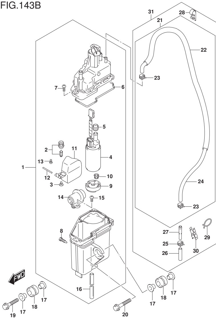
FIG.143B (1-C-8) FUEL VAPOR SEPARATOR (E40)
